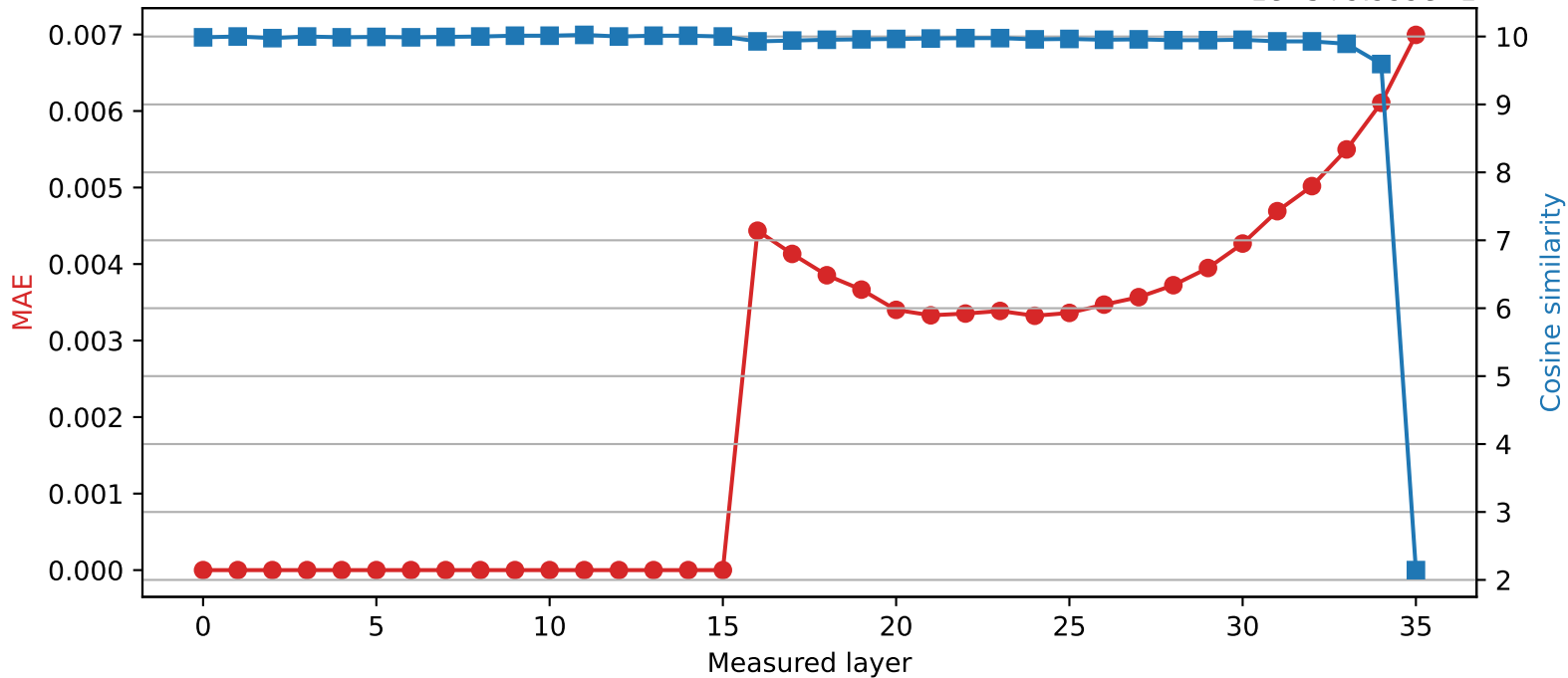
SmolLM3-3B | Quantized layer 15 | float16 → int8
