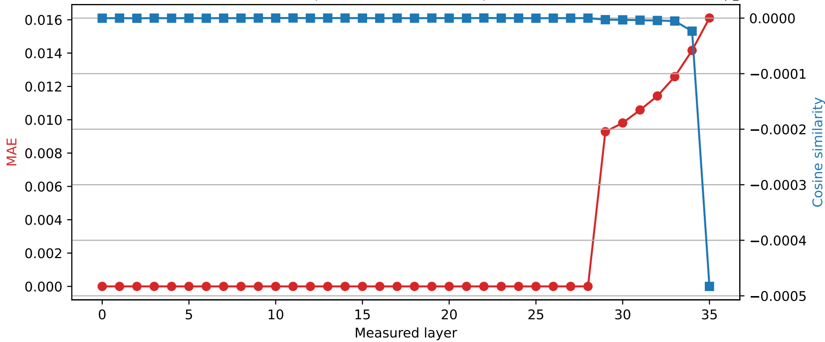
SmolLM3-3B | Quantized layer 28 | float16 \rightarrow int8
