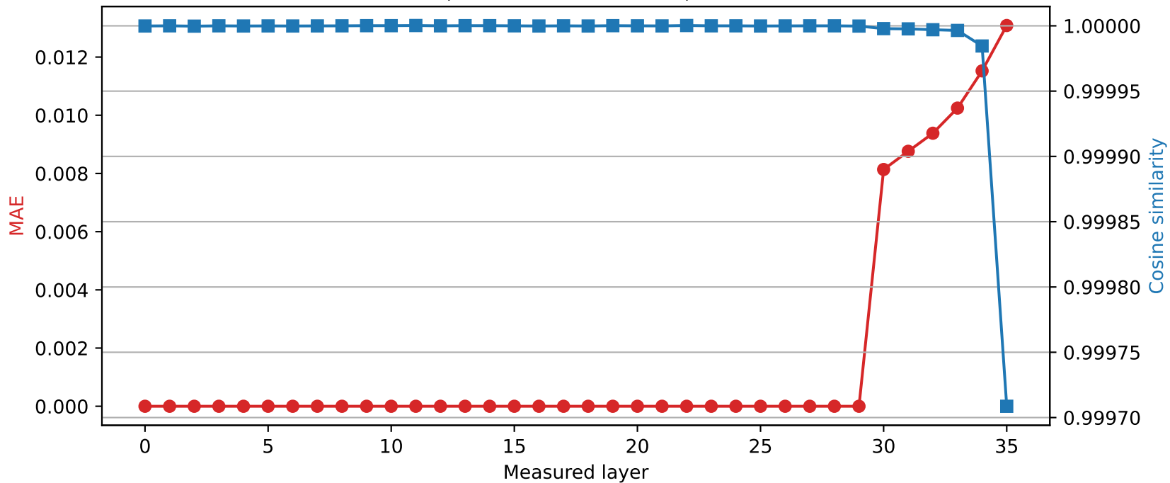
SmolLM3-3B | Quantized layer 29 | float16 → int8
