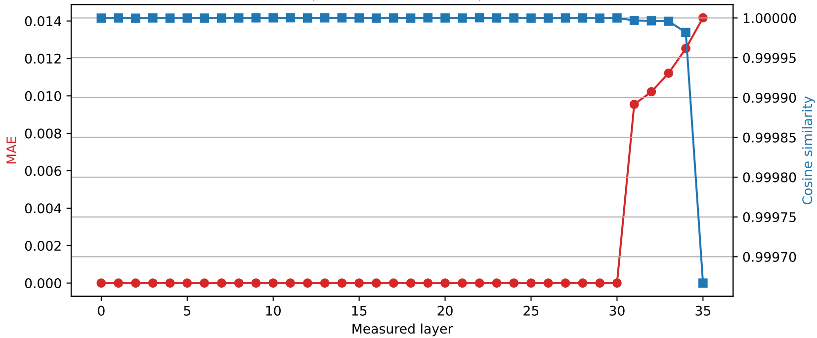
SmolLM3-3B | Quantized layer 30 | float16 \rightarrow int8
