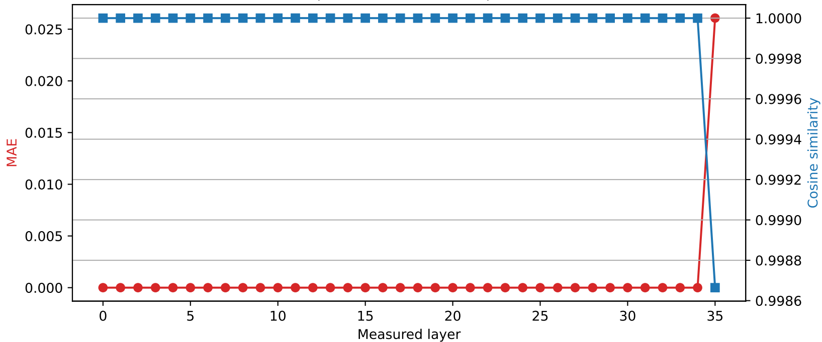
SmolLM3-3B | Quantized layer 34 | float16 → int8
