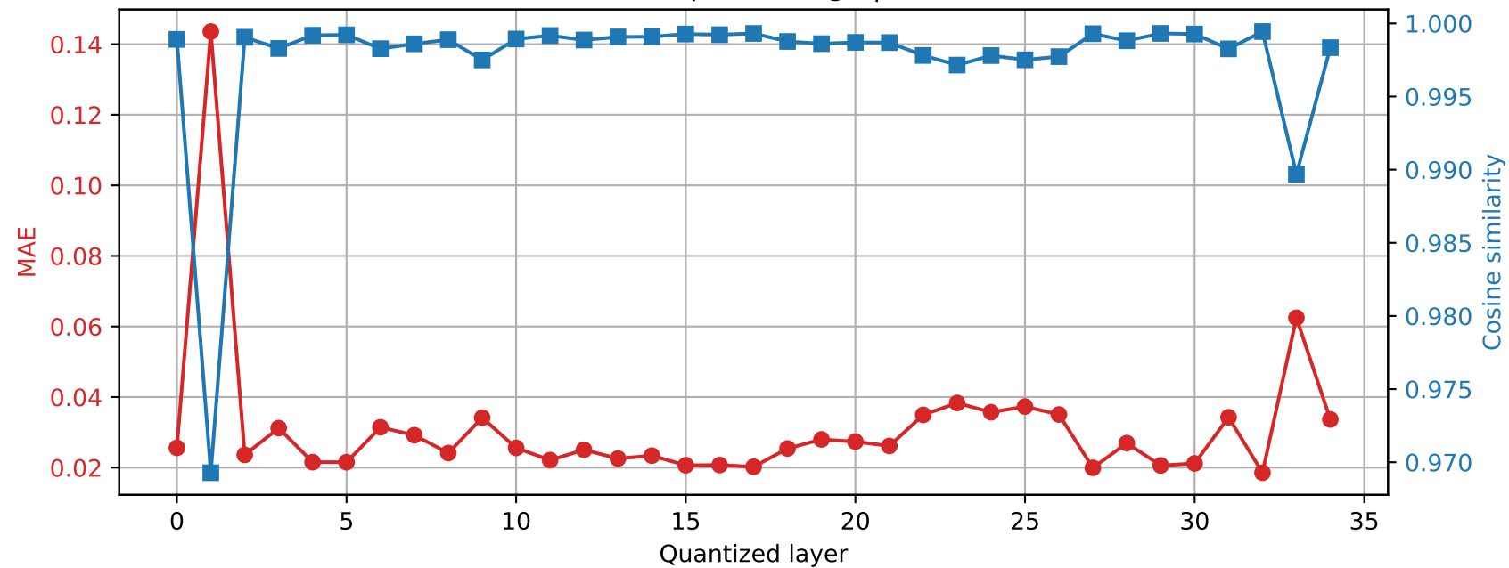
SmolLM3-3B | Prompt 3 Final RMSNorm output damage | float16 \rightarrow int8
