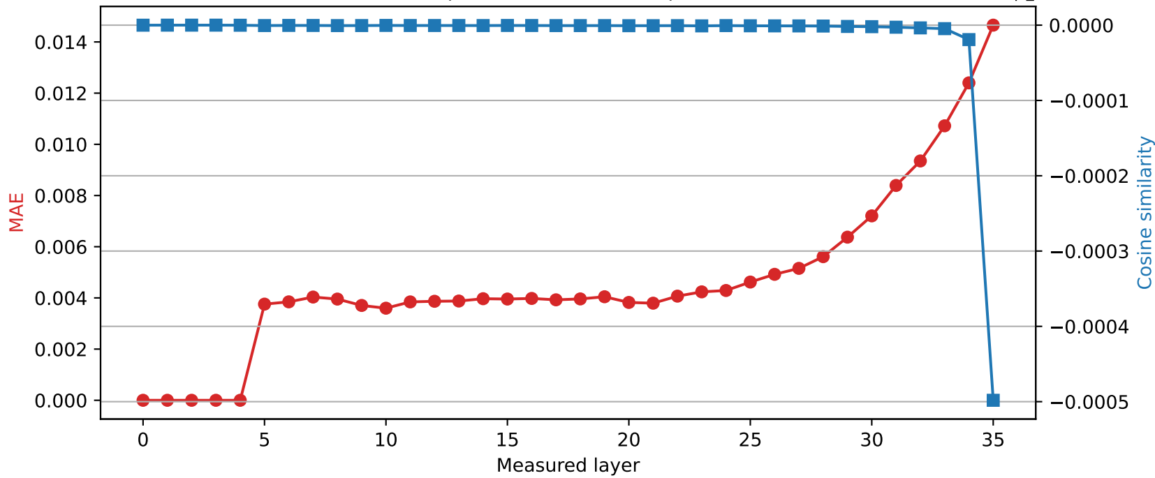
SmolLM3-3B | Quantized layer 4 | float16 → int8
