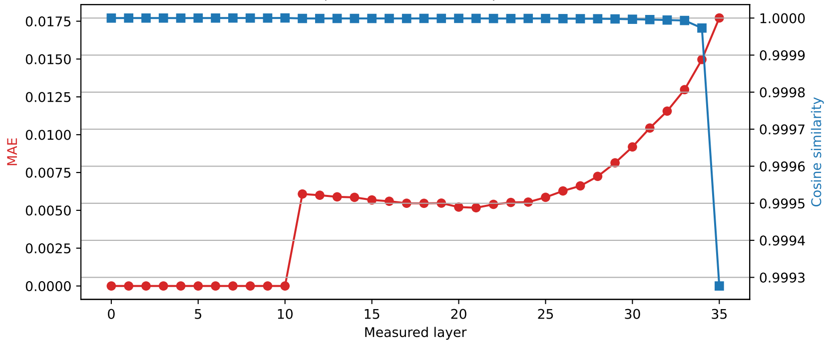
SmolLM3-3B | Quantized layer 10 | float16 → int8
