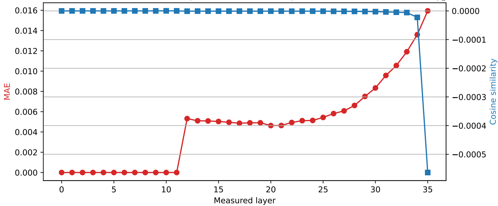
SmolLM3-3B | Quantized layer 11 | float16 \rightarrow int8
