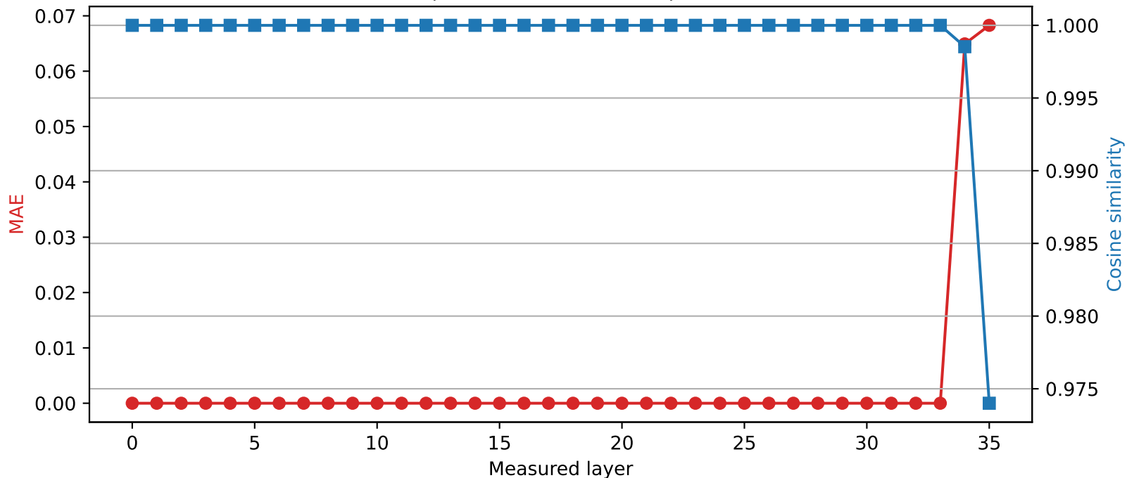
SmolLM3-3B | Quantized layer 33 | float16 \rightarrow int8
