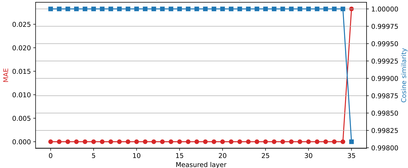
SmolLM3-3B | Quantized layer 34 | float16 \rightarrow int8
