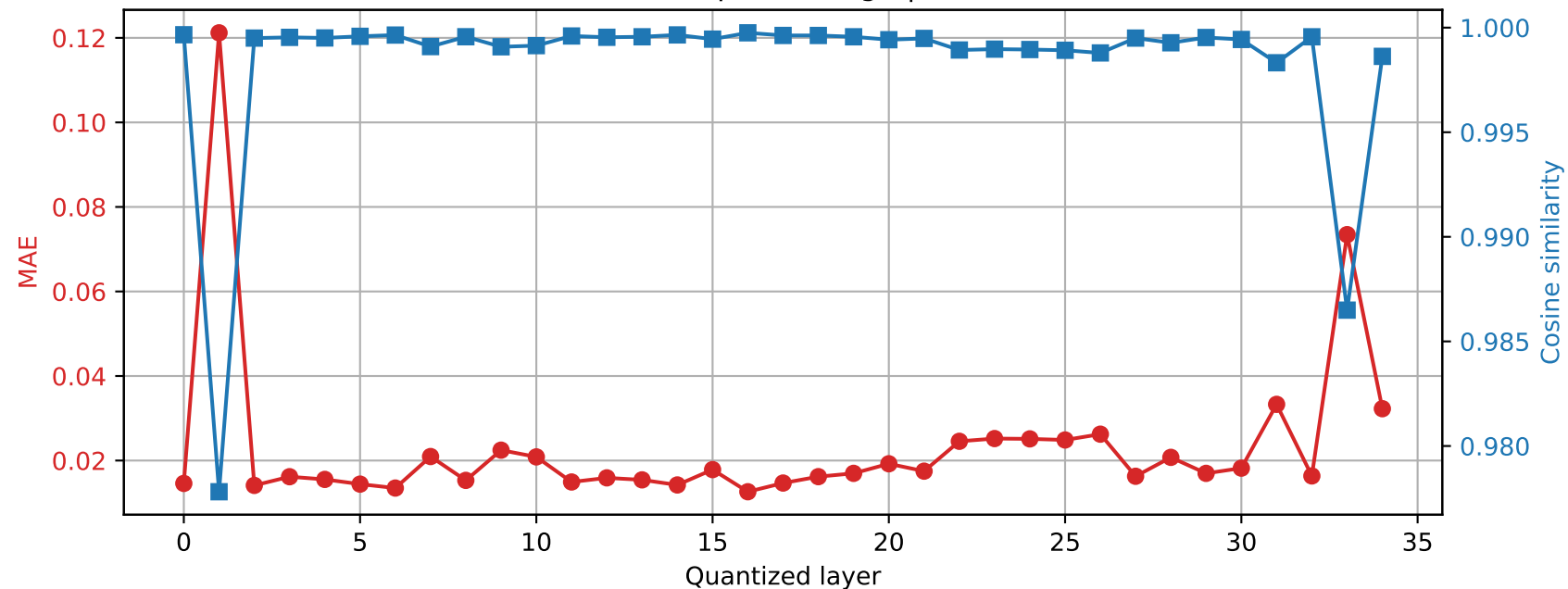
SmolLM3-3B | Prompt 4 Final RMSNorm output damage | float16 \rightarrow int8
