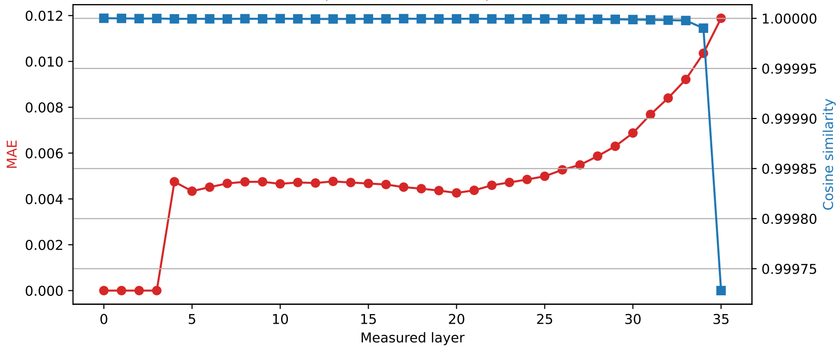
SmolLM3-3B | Quantized layer 3 | float16 → int8
