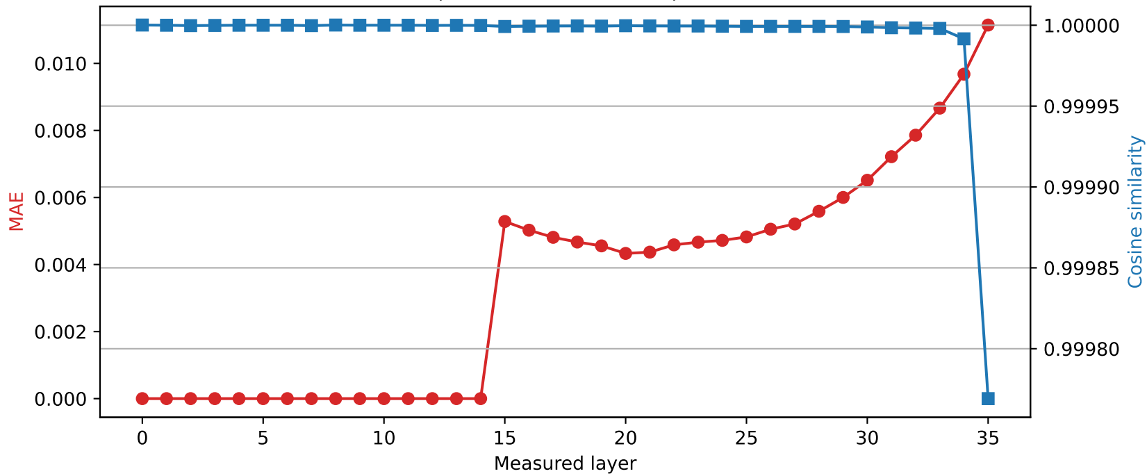
SmolLM3-3B | Quantized layer 14 | float16 \rightarrow int8
