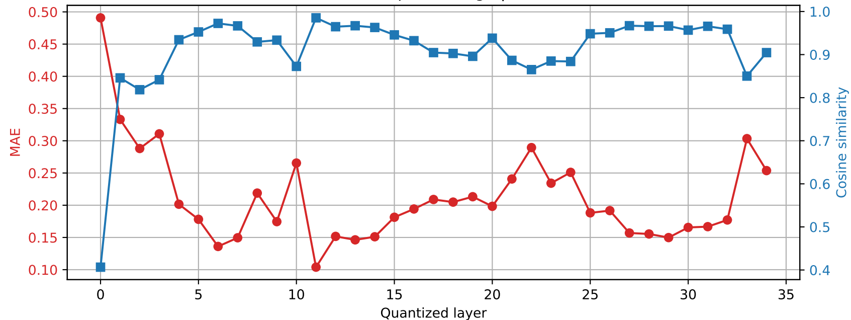
SmolLM3-3B | Prompt 0 Final RMSNorm output damage | float16 \rightarrow int4
