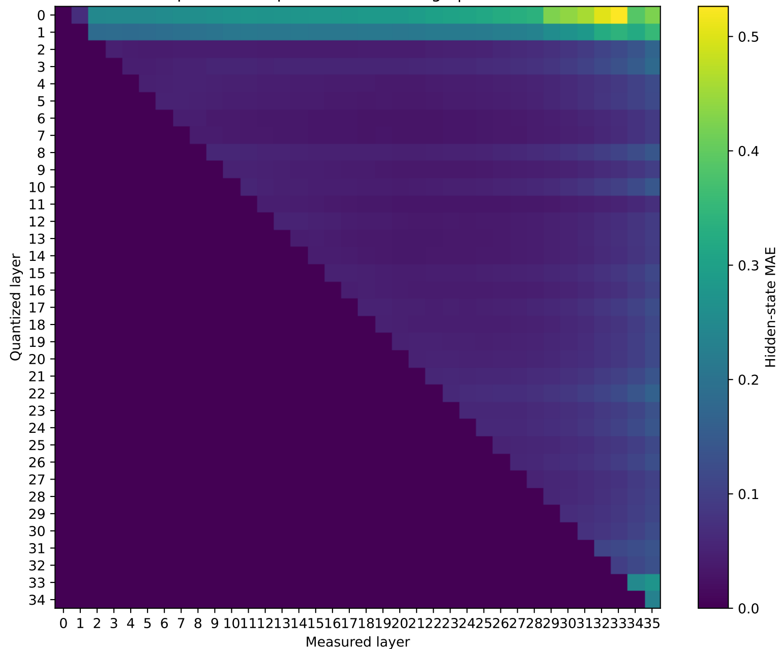
SmolLM3-3B Prompt 0: MAE representation damage | float16 → int4
