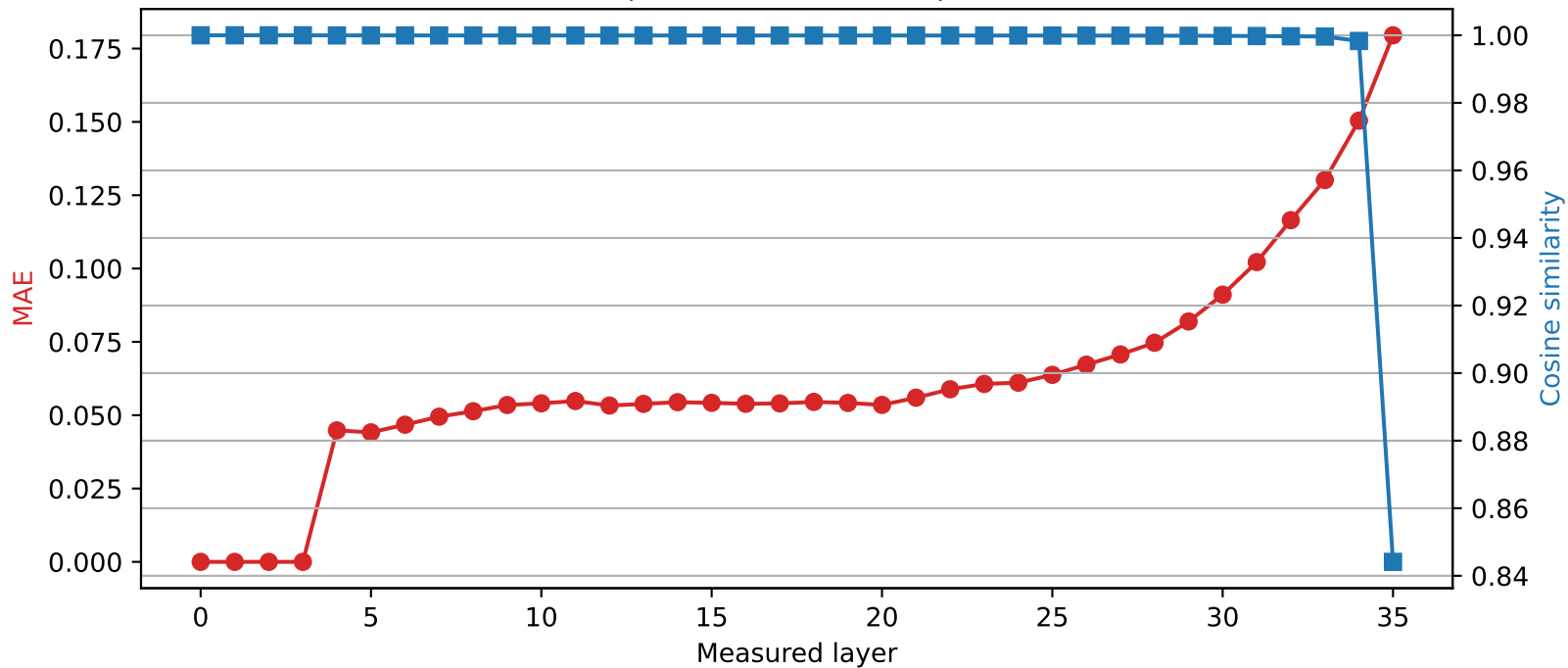
SmolLM3-3B | Quantized layer 3 | float16 → int4
