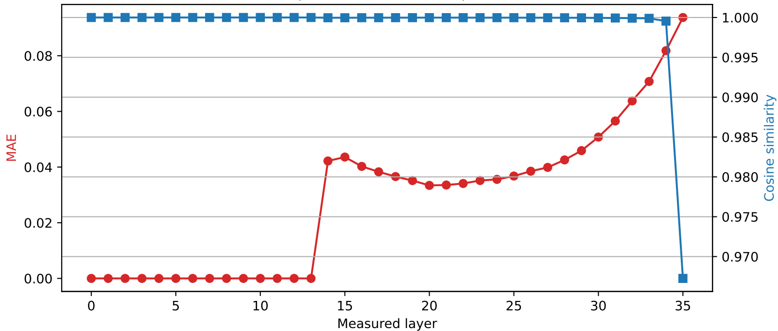
SmolLM3-3B | Quantized layer 13 | float16 \rightarrow int4
