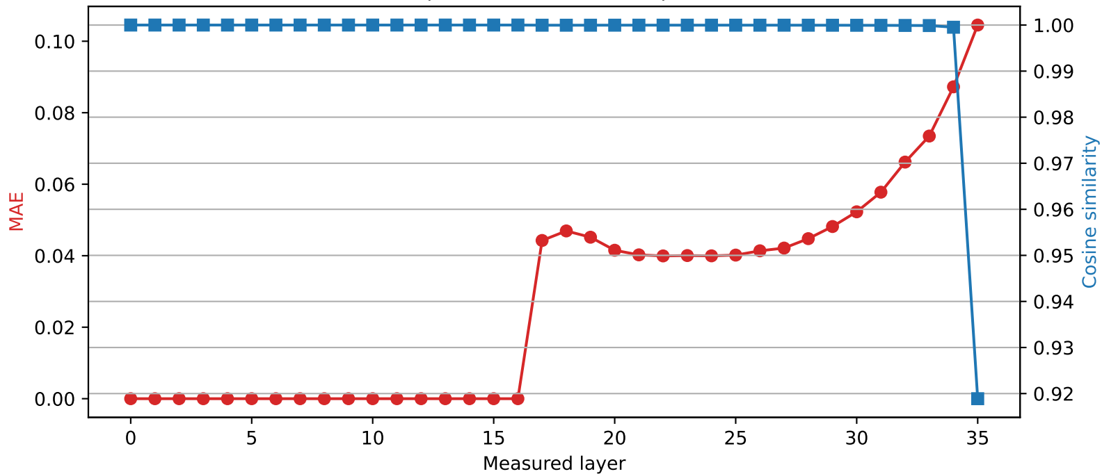
SmolLM3-3B | Quantized layer 16 | float16 → int4
