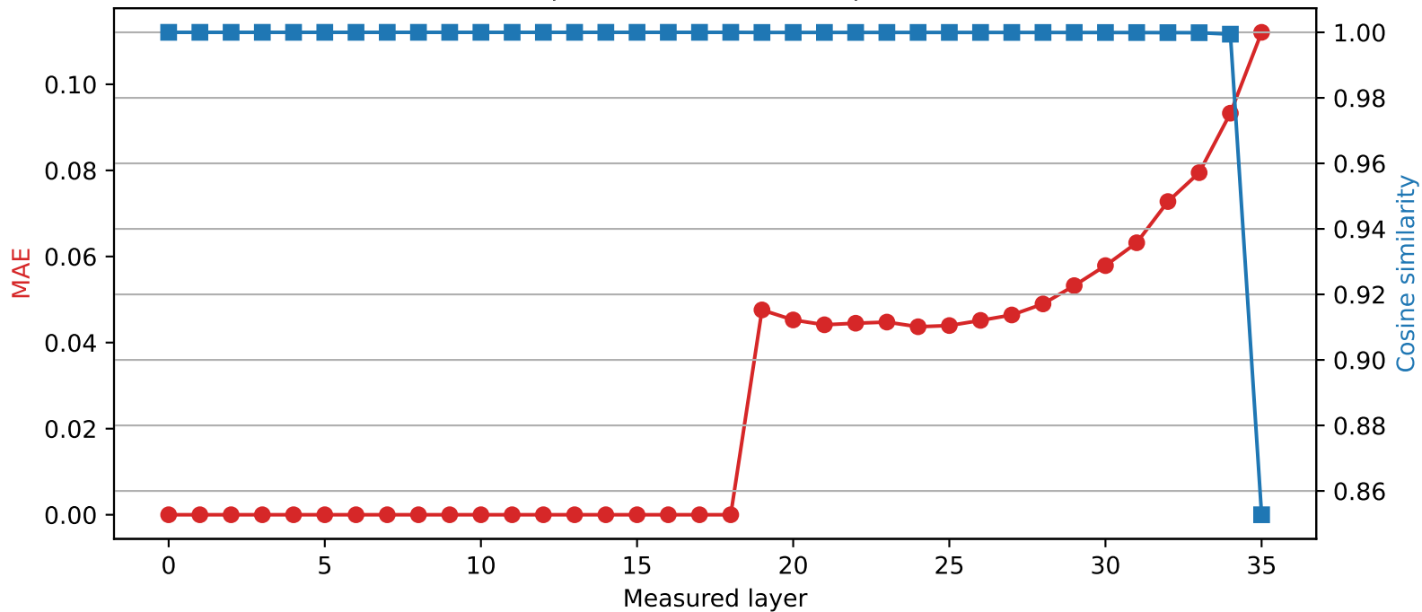
SmolLM3-3B | Quantized layer 18 | float16 \rightarrow int4
