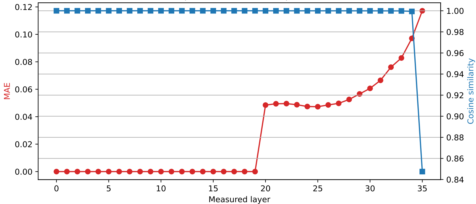
SmolLM3-3B | Quantized layer 19 | float16 \rightarrow int4
