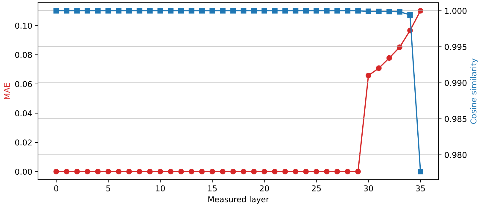
SmolLM3-3B | Quantized layer 29 | float16 \rightarrow int4
