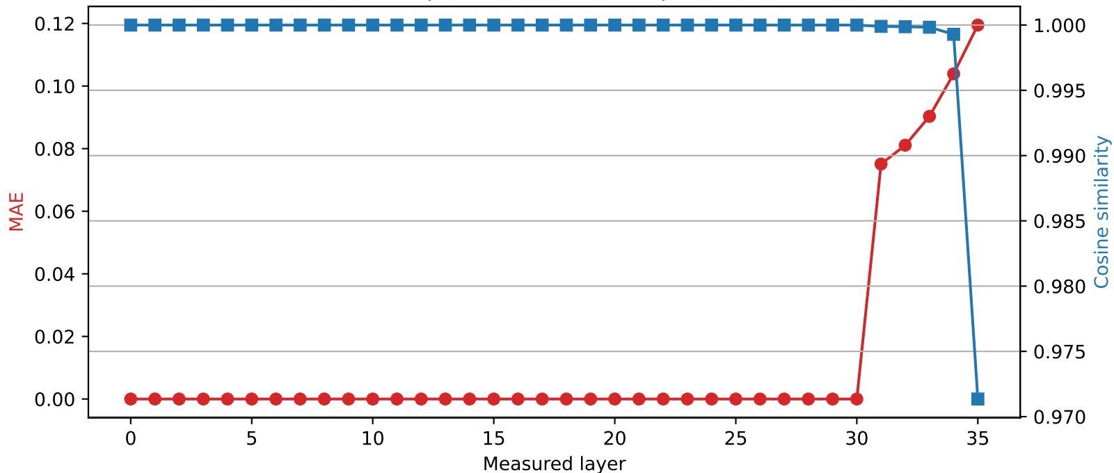
SmolLM3-3B | Quantized layer 30 | float16 \rightarrow int4
