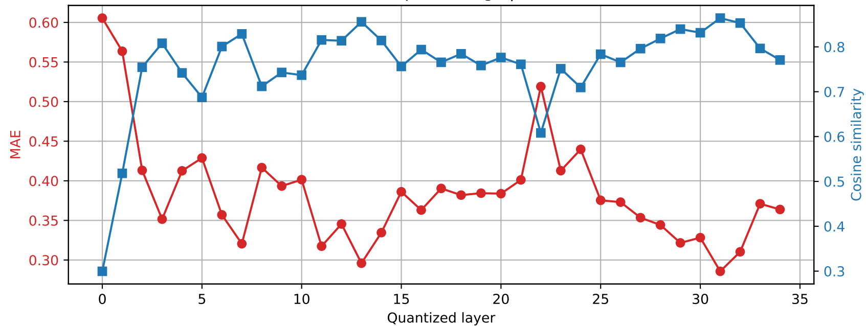
SmolLM3-3B | Prompt 1 Final RMSNorm output damage | float16 \rightarrow int4
