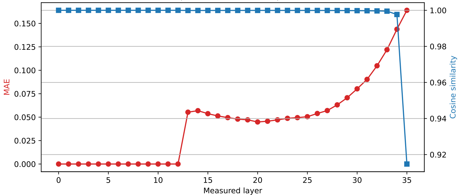
SmolLM3-3B | Quantized layer 12 | float16 \rightarrow int4
