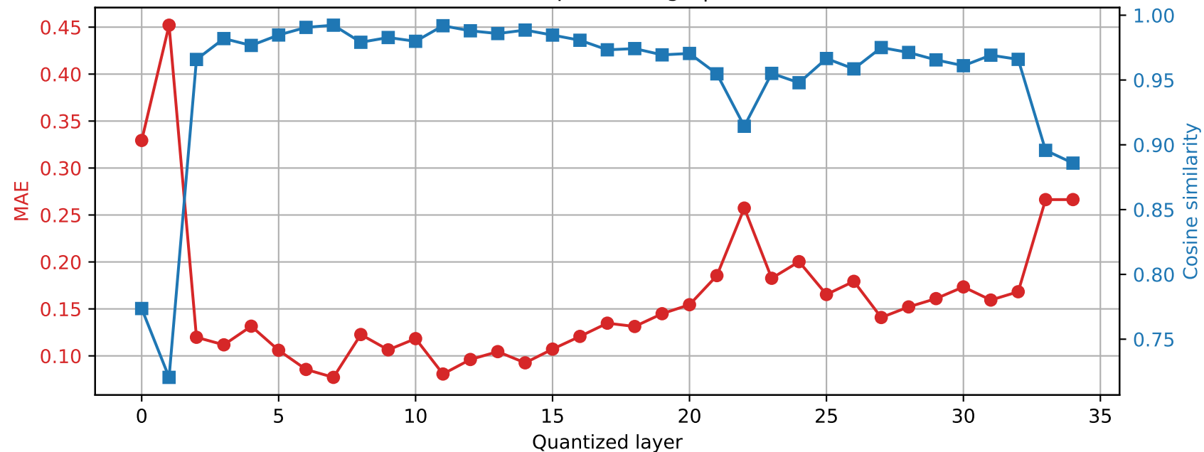
SmolLM3-3B | Prompt 2 Final RMSNorm output damage | float16 \rightarrow int4
