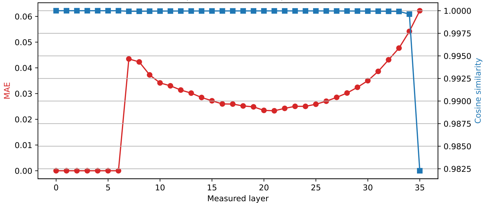
SmolLM3-3B | Quantized layer 6 | float16 → int4
