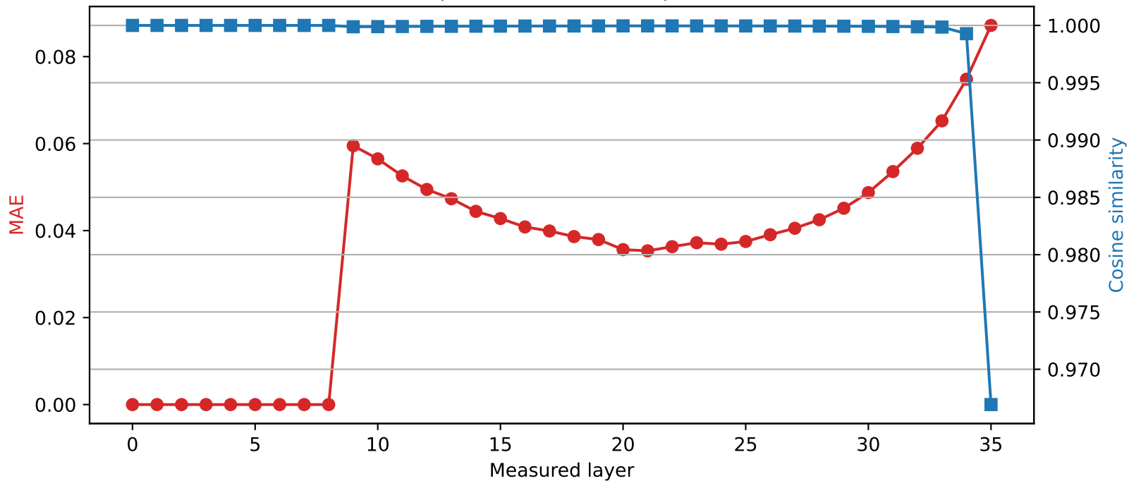
SmolLM3-3B | Quantized layer 8 | float16 → int4
