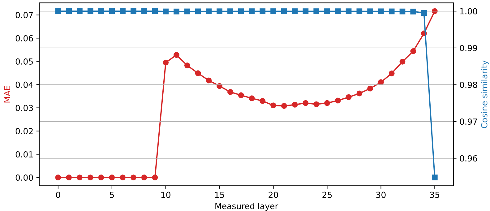
SmolLM3-3B | Quantized layer 9 | float16 \rightarrow int4
