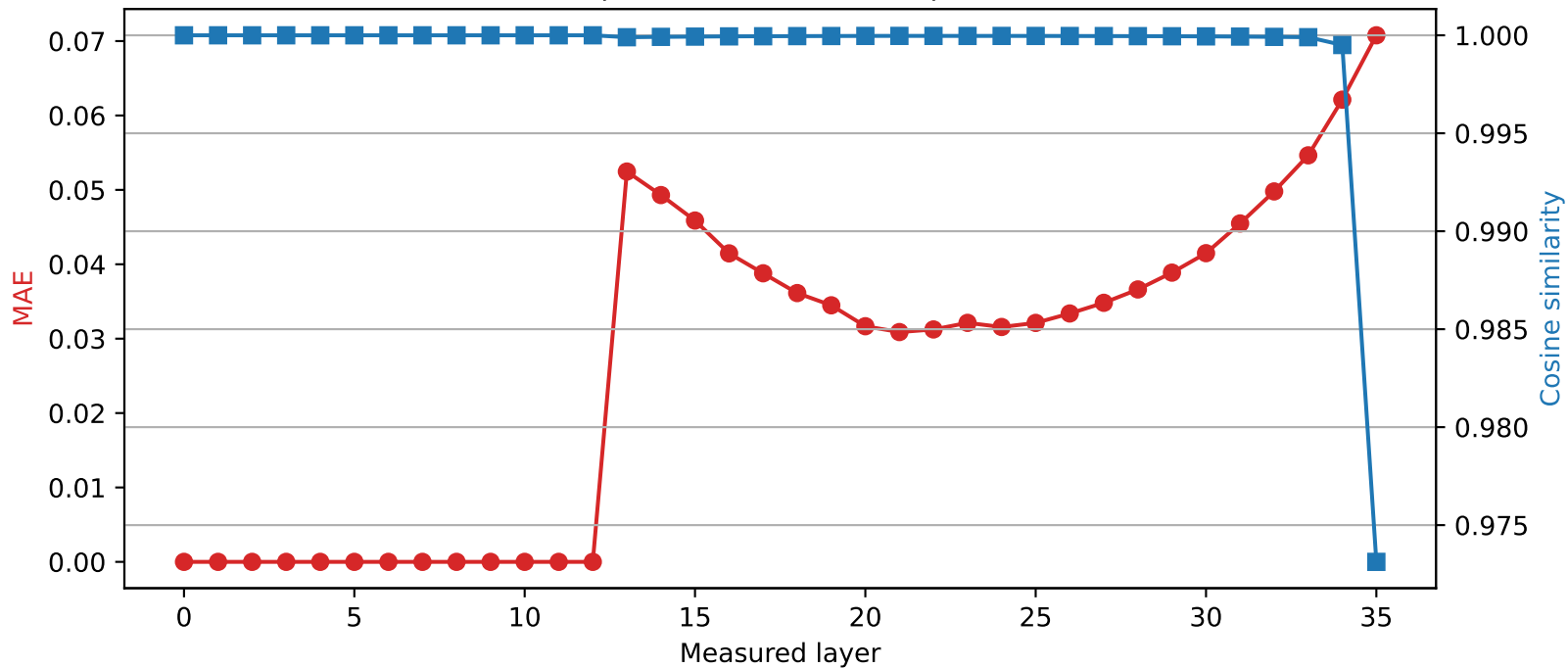
SmolLM3-3B | Quantized layer 12 | float16 → int4
