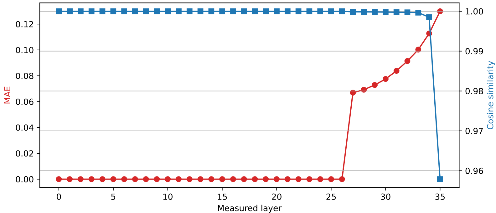
SmolLM3-3B | Quantized layer 26 | float16 \rightarrow int4
