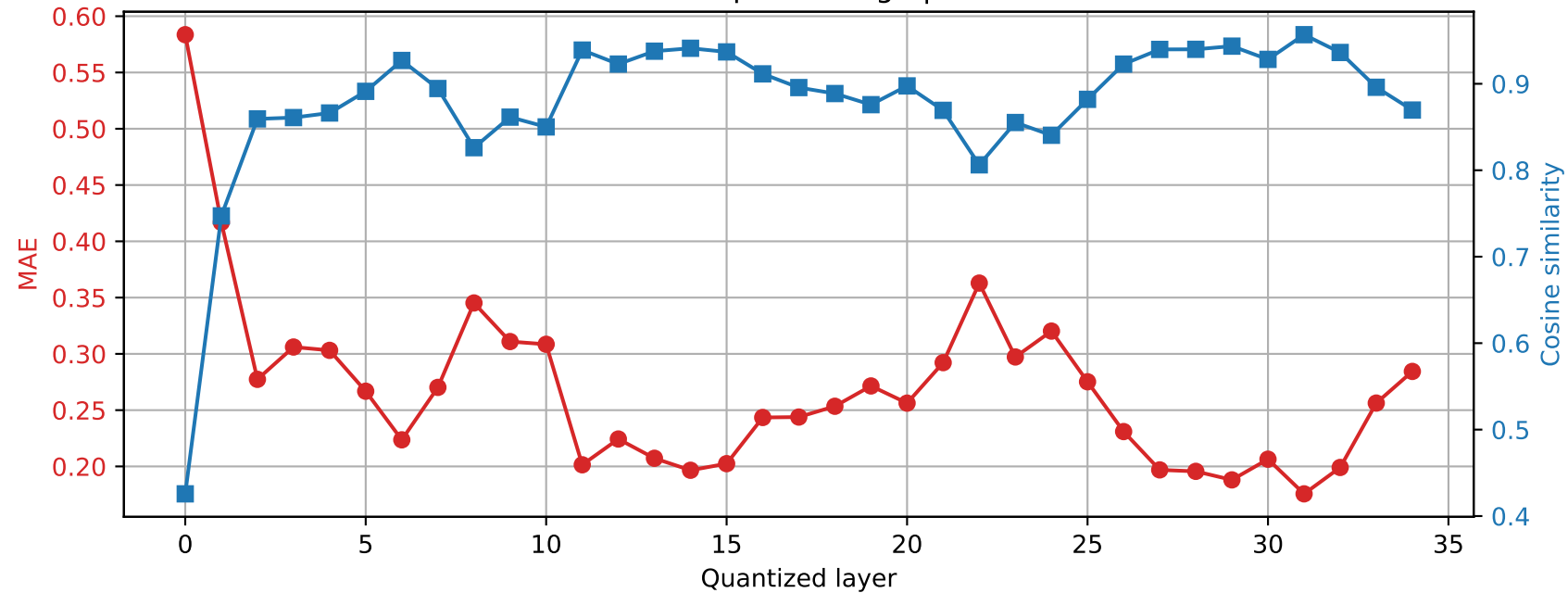
SmolLM3-3B | Prompt 3 Final RMSNorm output damage | float16 \rightarrow int4
