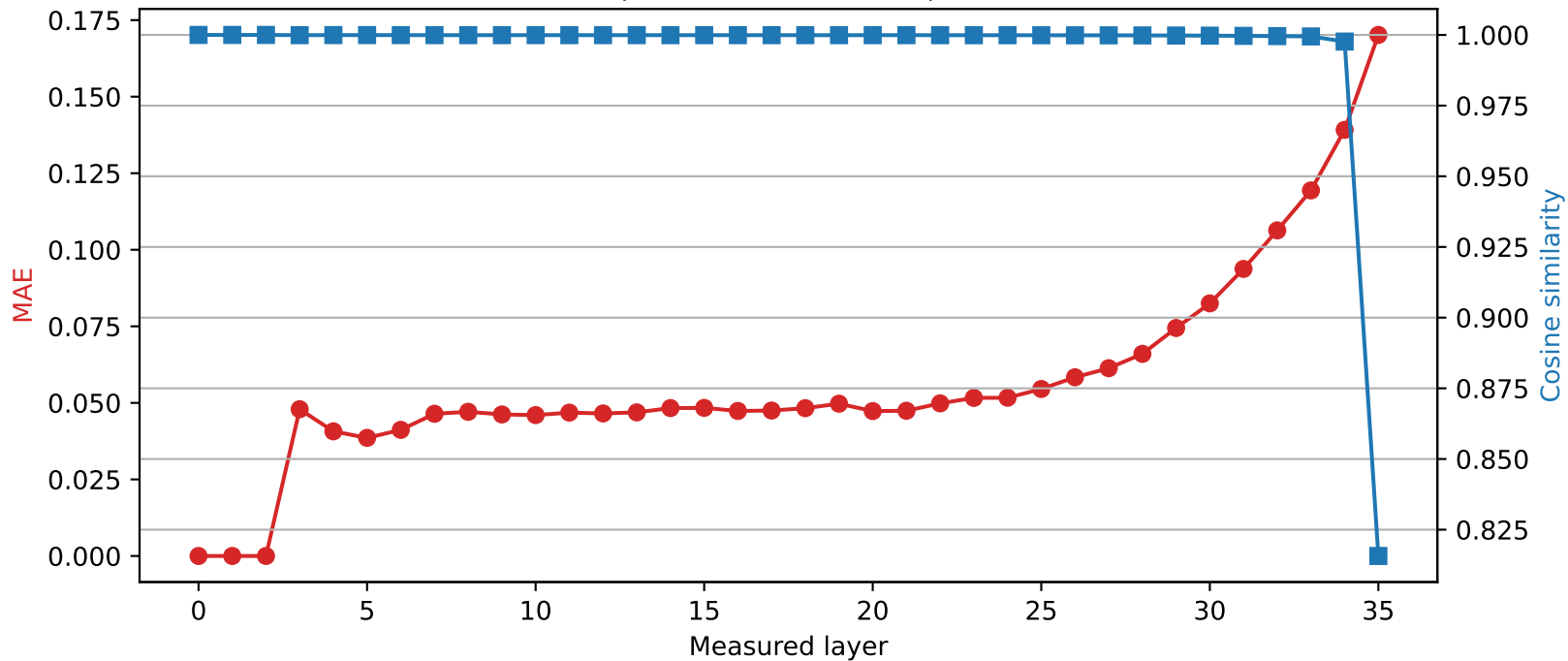
SmolLM3-3B | Quantized layer 2 | float16 \rightarrow int4
