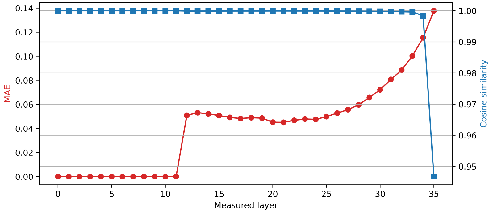
SmolLM3-3B | Quantized layer 11 | float16 \rightarrow int4
