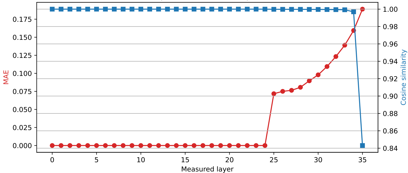
SmolLM3-3B | Quantized layer 24 | float16 → int4
