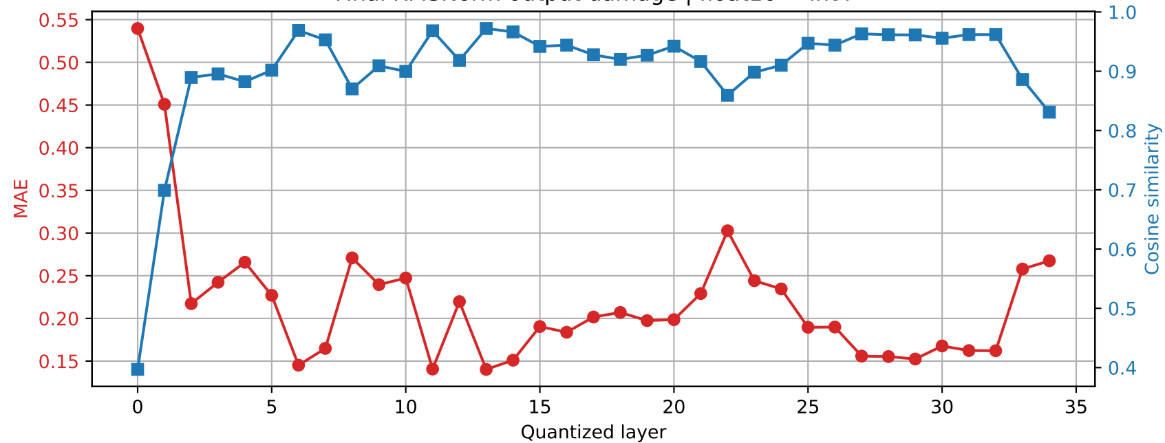
SmolLM3-3B | Prompt 4 Final RMSNorm output damage | float16 \rightarrow int4
