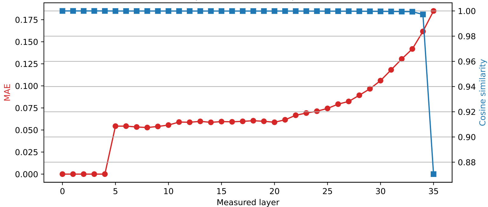
SmolLM3-3B | Quantized layer 4 | float16 → int4
