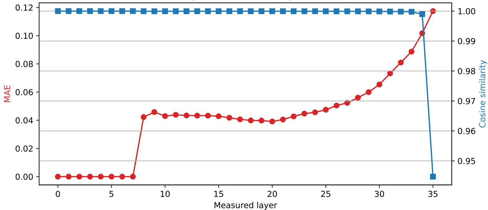
SmolLM3-3B | Quantized layer 7 | float16 \rightarrow int4
