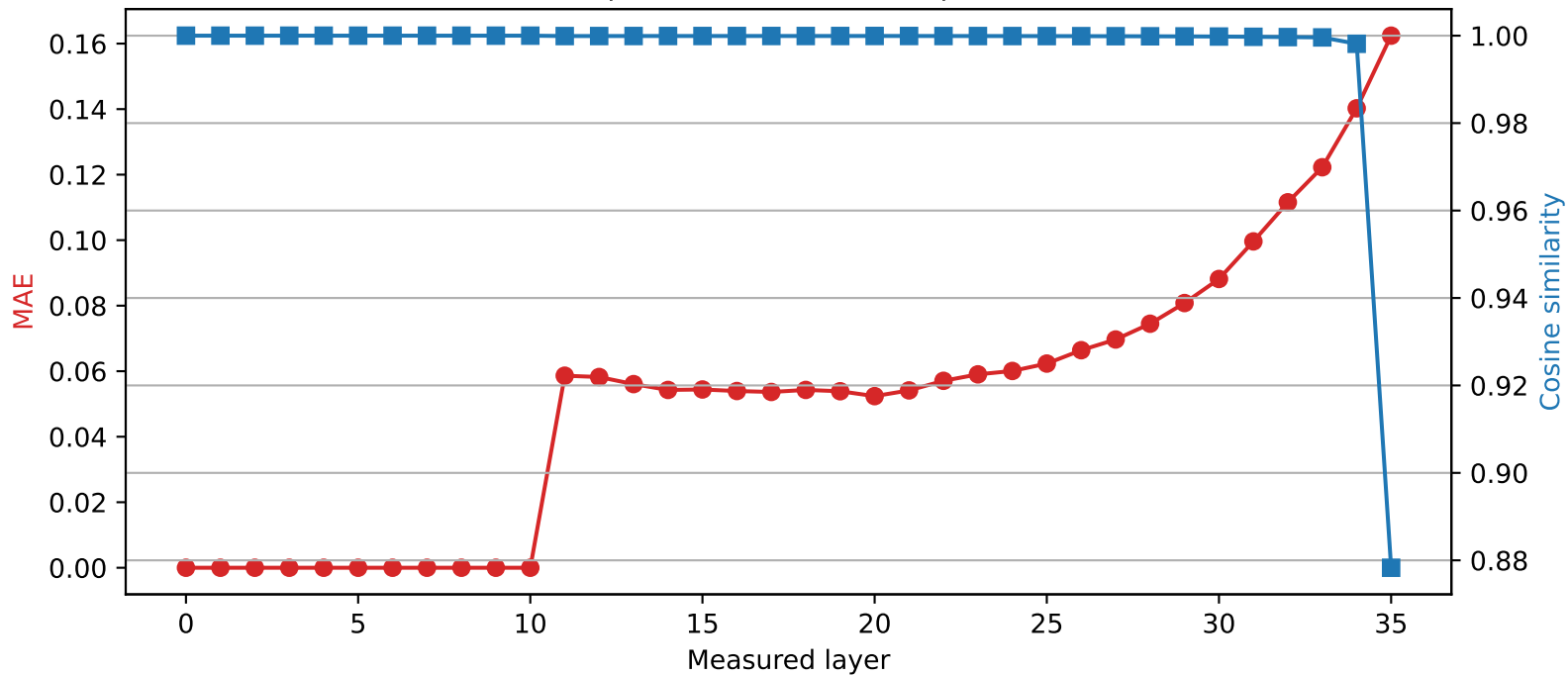
SmolLM3-3B | Quantized layer 10 | float16 \rightarrow int4
