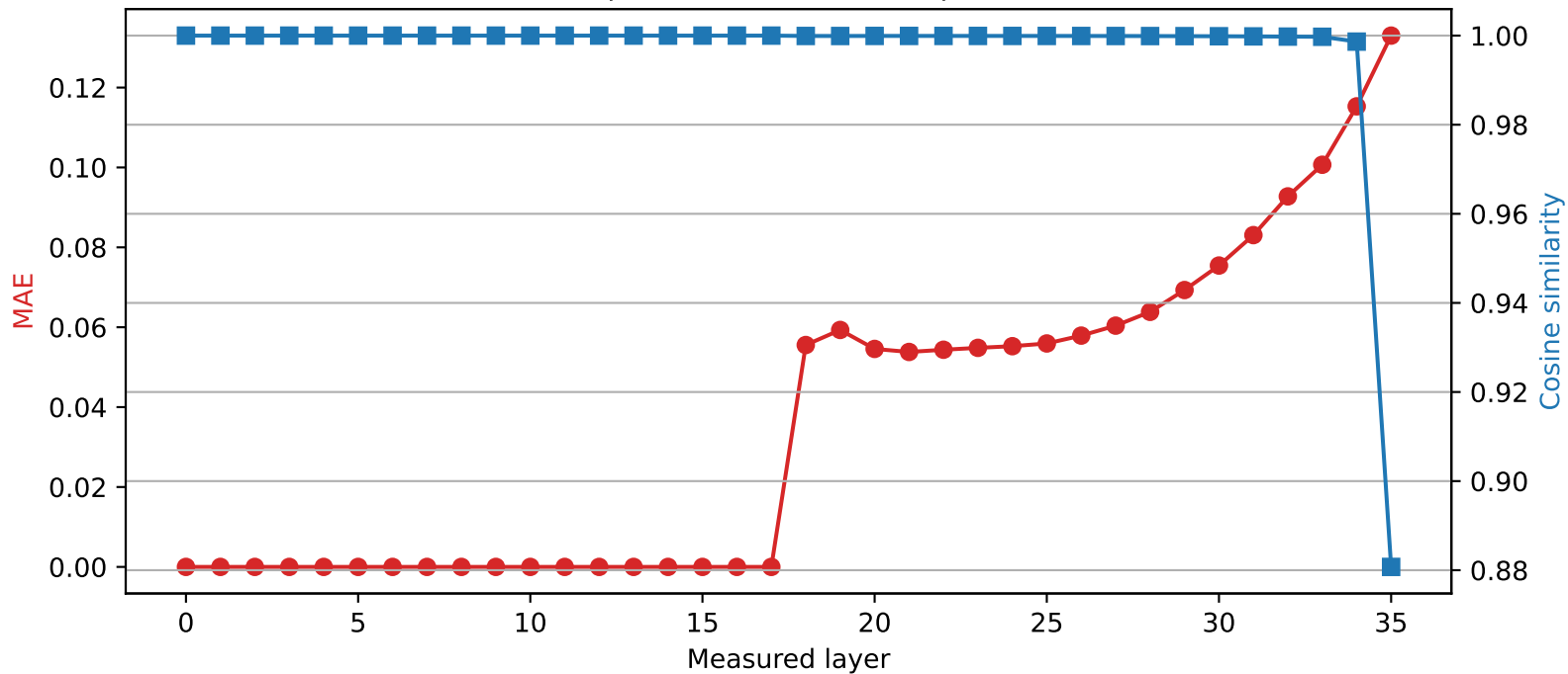
SmolLM3-3B | Quantized layer 17 | float16 \rightarrow int4
