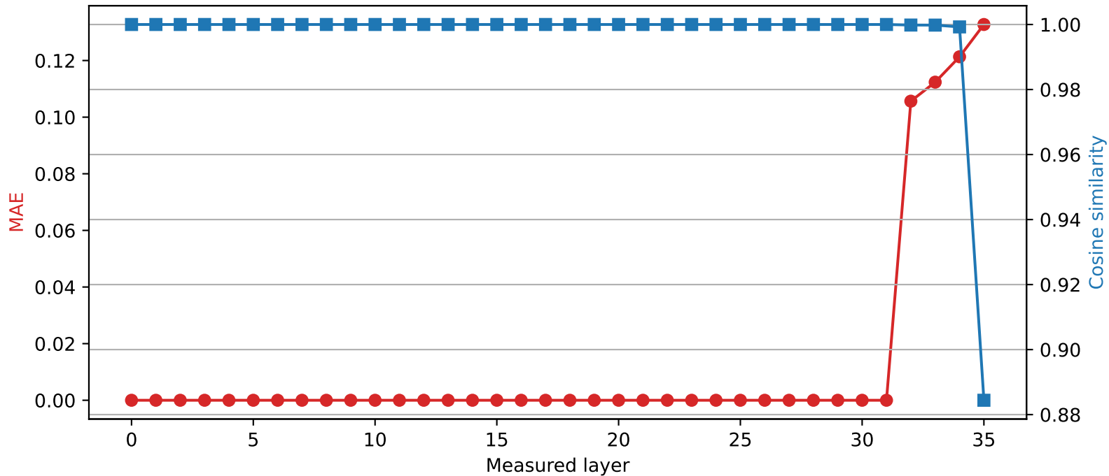
SmolLM3-3B | Quantized layer 31 | float16 \rightarrow int2
