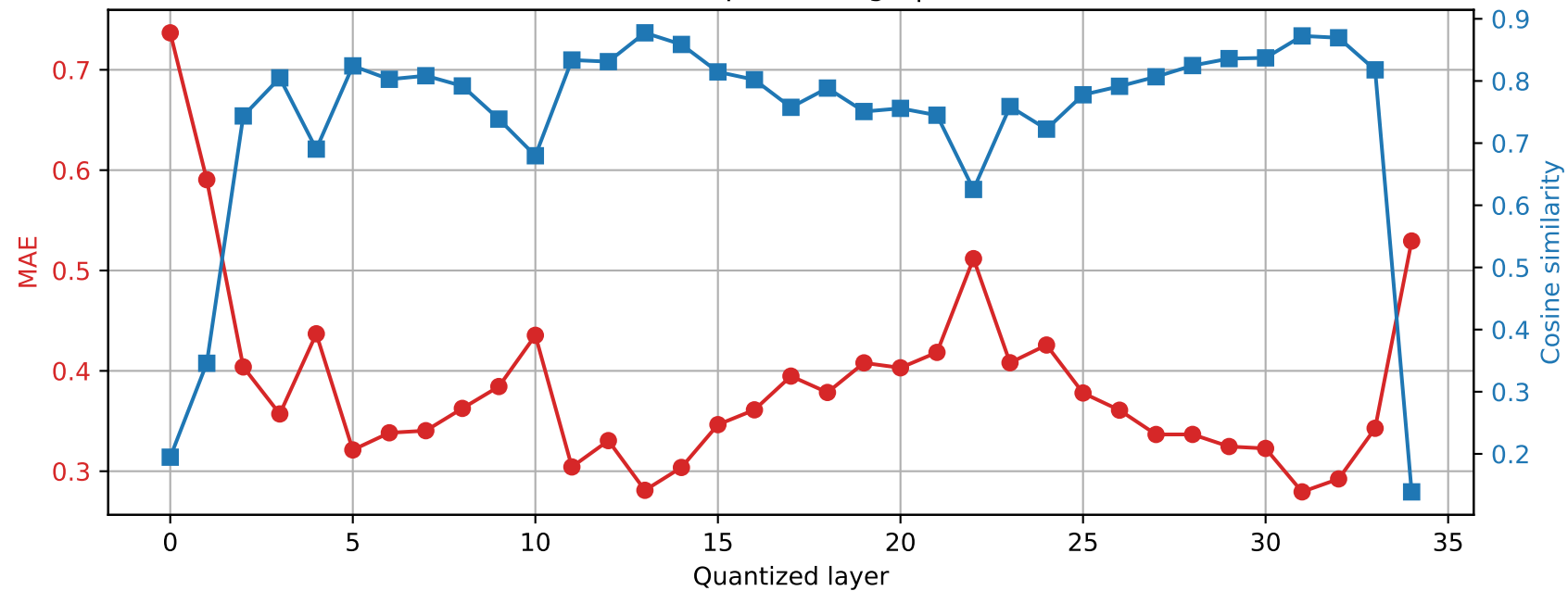
SmolLM3-3B | Prompt 1 Final RMSNorm output damage | float16 \rightarrow int2
