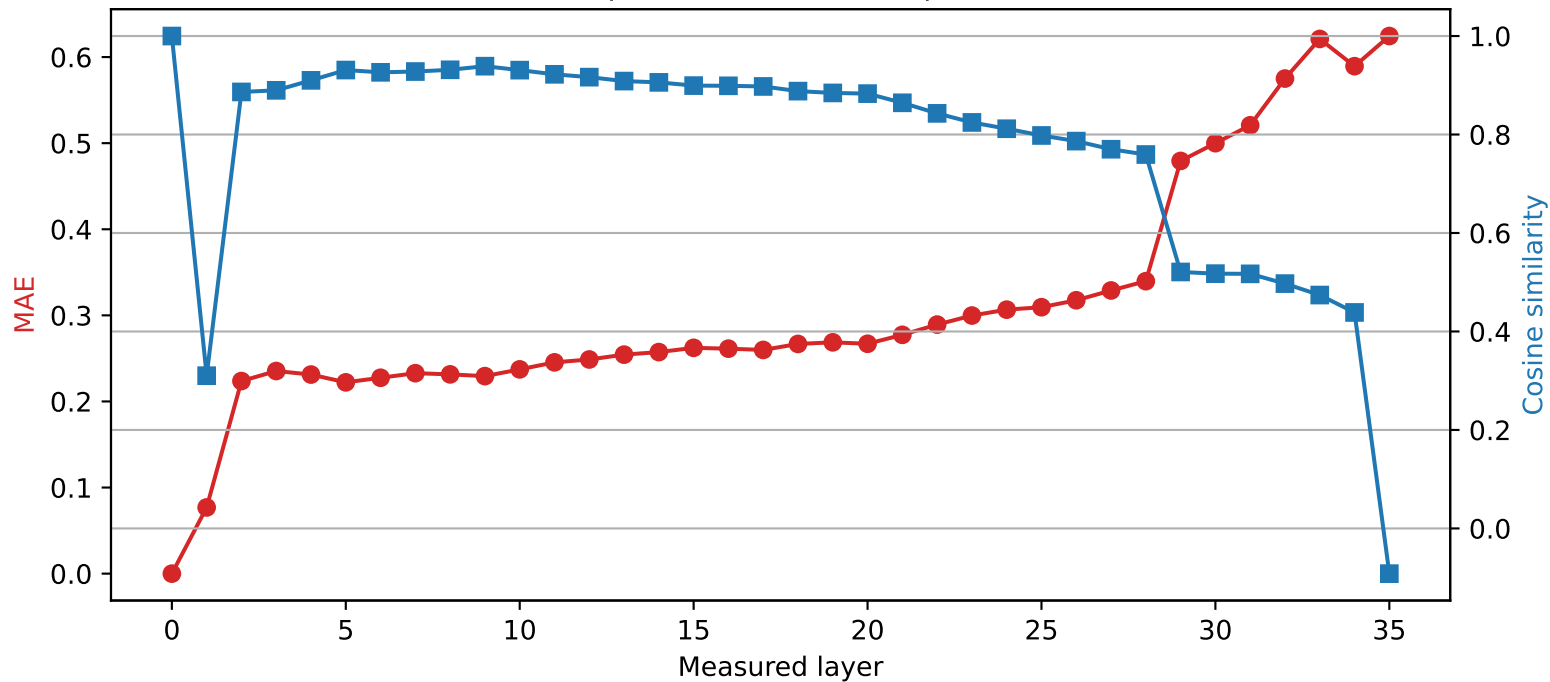
SmolLM3-3B | Quantized layer 0 | float16 → int2
