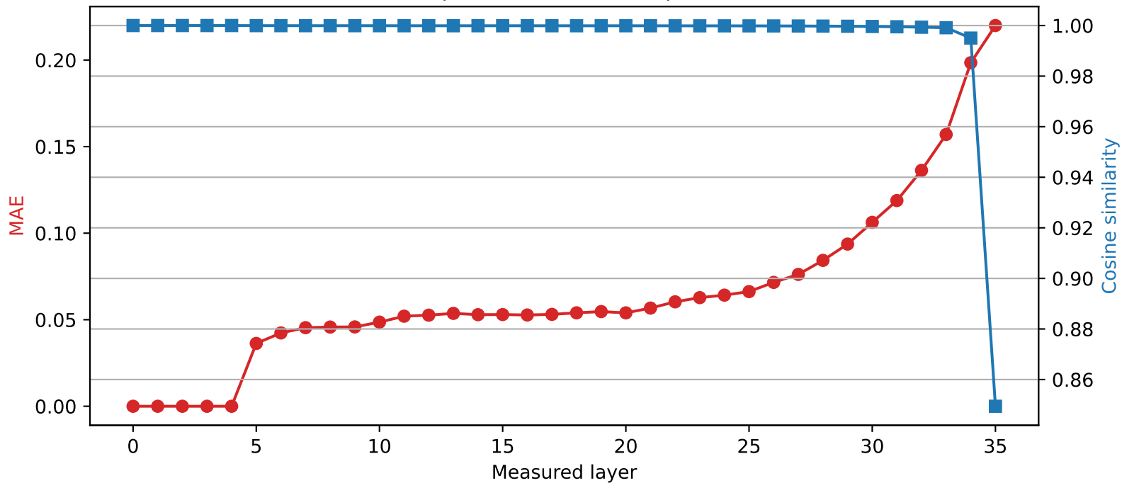
SmolLM3-3B | Quantized layer 4 | float16 \rightarrow int2
