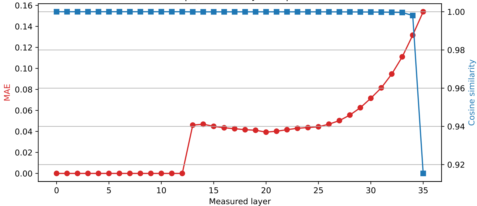
SmolLM3-3B | Quantized layer 12 | float16 \rightarrow int2
