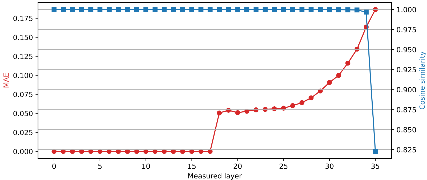
SmolLM3-3B | Quantized layer 17 | float16 \rightarrow int2
