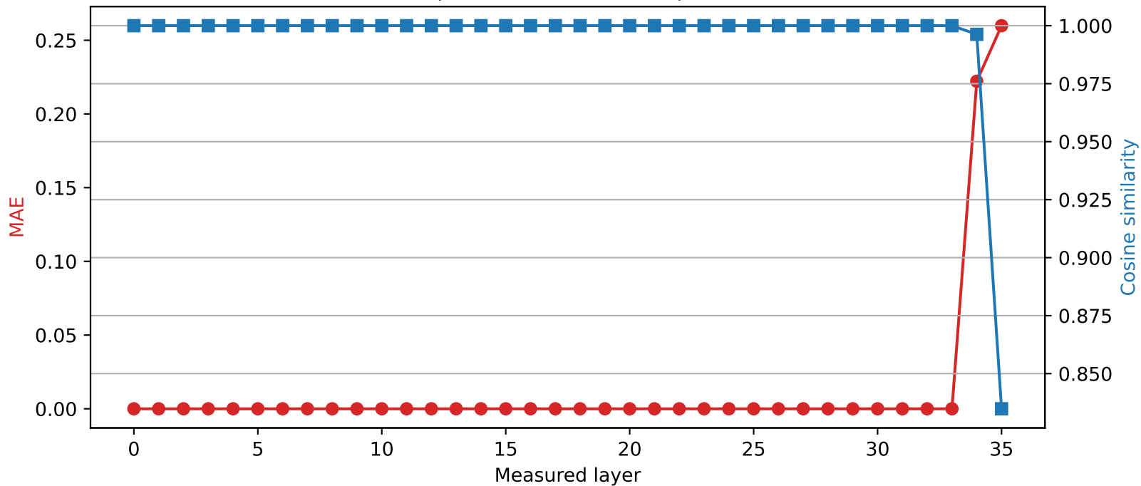
SmolLM3-3B | Quantized layer 33 | float16 \rightarrow int2
