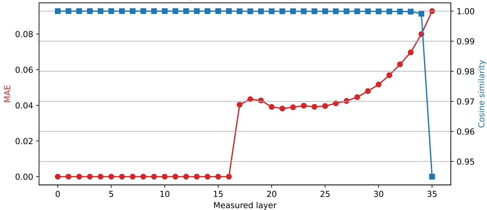
SmolLM3-3B | Quantized layer 16 | float16 → int2
