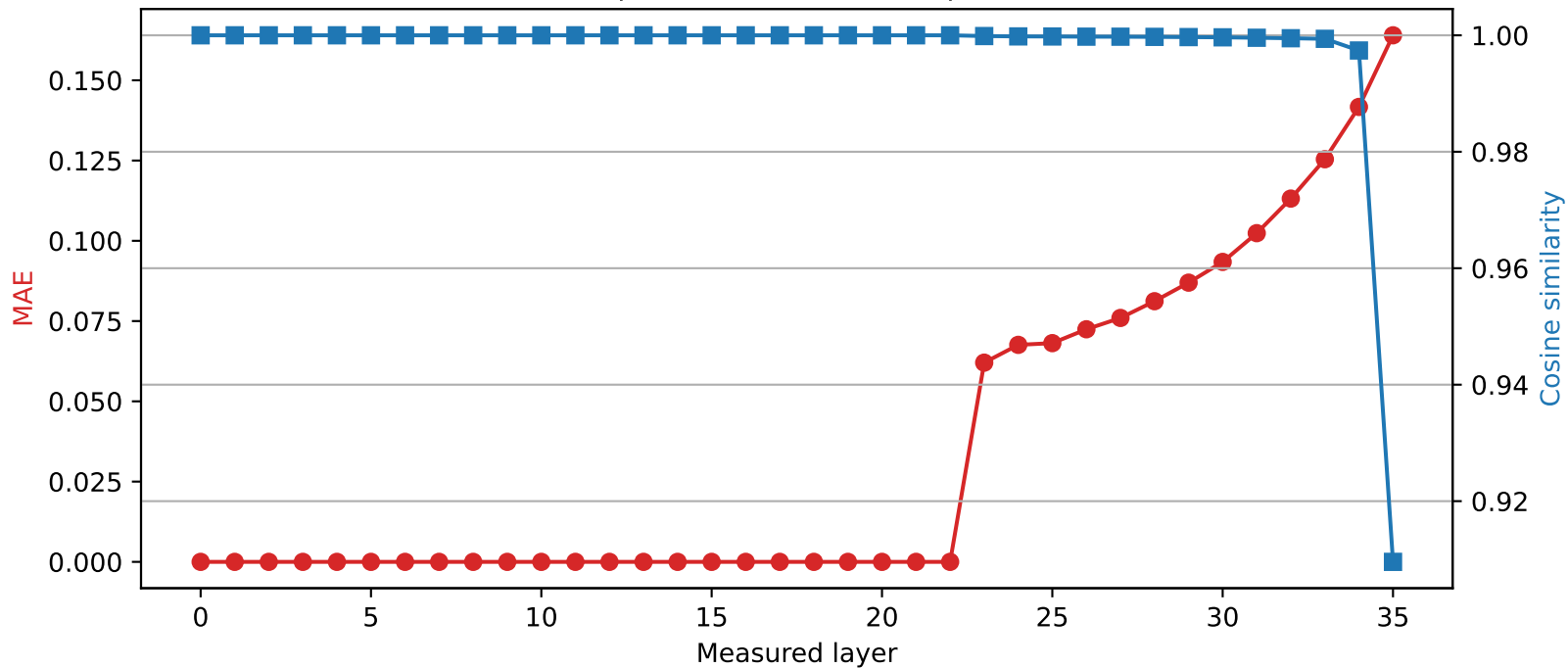
SmolLM3-3B | Quantized layer 22 | float16 \rightarrow int2
