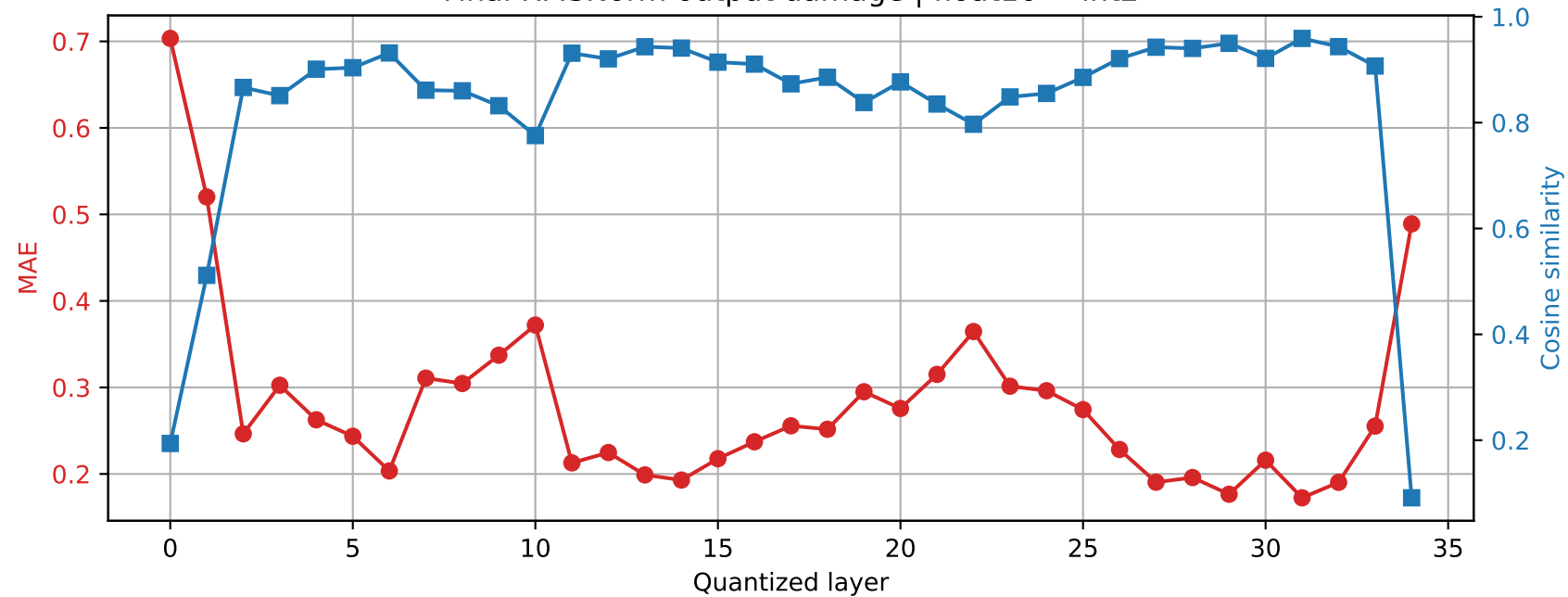
SmolLM3-3B | Prompt 3 Final RMSNorm output damage | float16 \rightarrow int2
